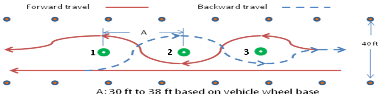
Figure A-4.3.3 Serpentine Exercise. (Minimum 9 traffic cones) Copyright NFPA
