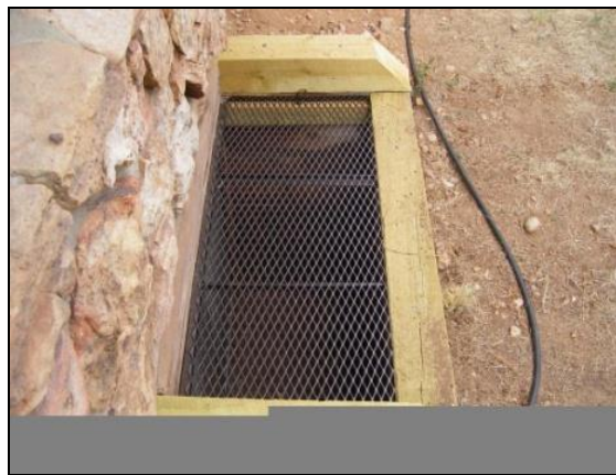
Figure 48. Appropriate Window Well Screening
