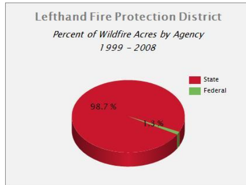
Figure 27. LHFPD Percent of Wildfire by Agency (Number and Acres)
