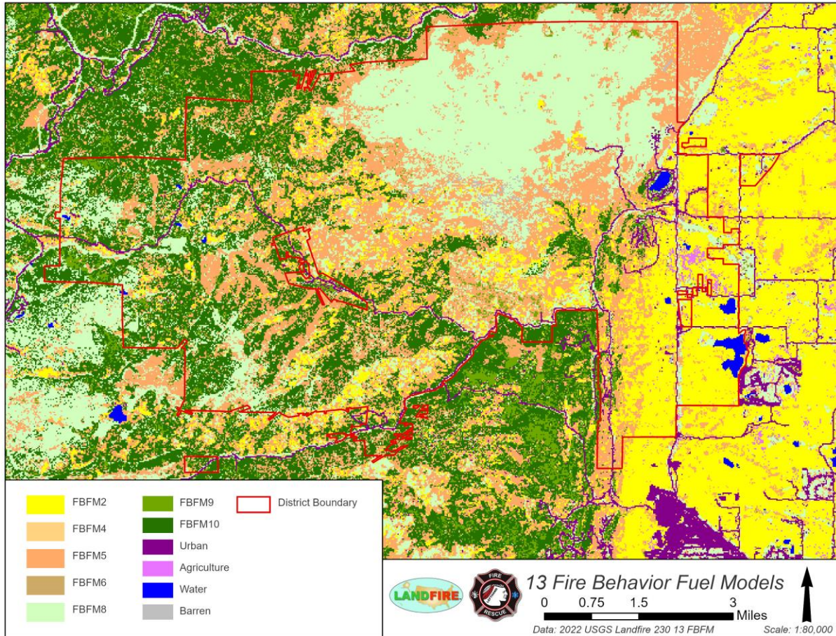
Figure 18. Anderson fuel models within and adjacent to Lefthand Fire Protection District
